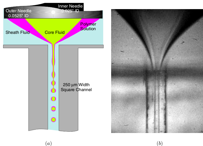
Figure 2. Schematic diagram (a) and photo (b) of the hydrodynamic focusing region and the compound jet formation. Note: \sim 2 mm from the microchannel inlet was obscured later in the experiment to secure the leakage.
