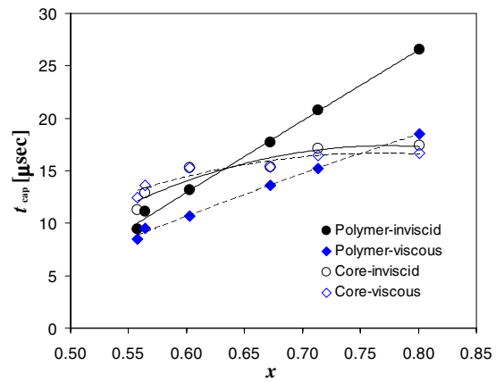
Figure 7. Capillary time of the compound jet with respect to the reduced wave number, x = \pi d_j/\lambda . ● and ○ are the inviscid capillary times, t_{\text{cap}} = (\rho r_j^3/\gamma)^{1/2} , for the polymer solution and the core fluid, respectively. ◆ and ◇ are the viscous capillary times, t_{\text{cap}} = C\mu r_j/\gamma , for the polymer solution and the core fluid, respectively. Note: for polymer solution, the jet radius of (r_{j,p} - r_{j,c}) has been used.
